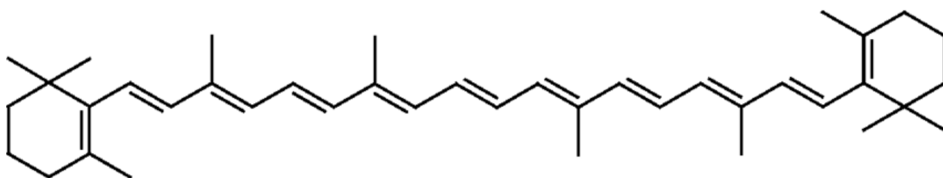
β-Carotene
