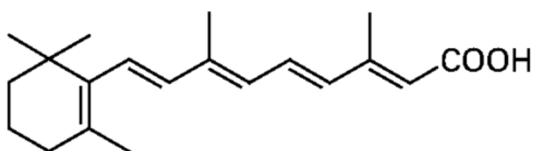
All-trans-retinoic acid
