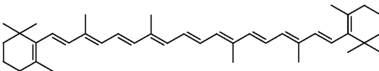
β-Carotene
